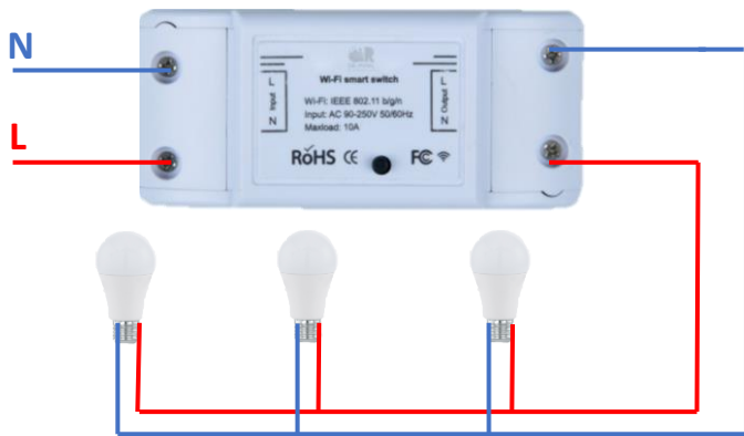
a. Ceiling lamp wiring instruction
